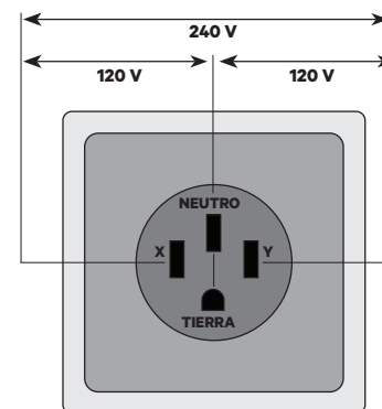
14-50R Tomacorriente "RV" 240 V/50 A
